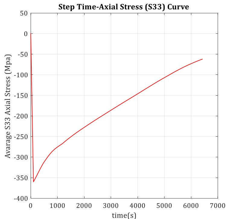
Fig. 10. Variation of axial stresses S33 in the bolt shank (avg.).
