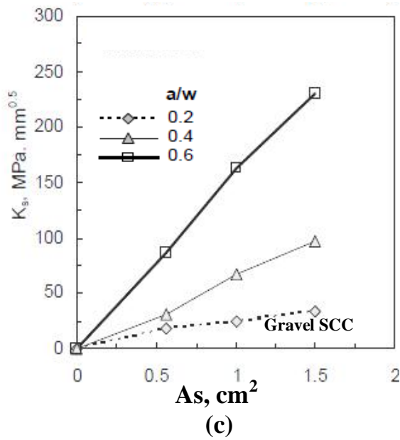
Fig. 7 Effect of area of steel on the closing SIF of SCC
