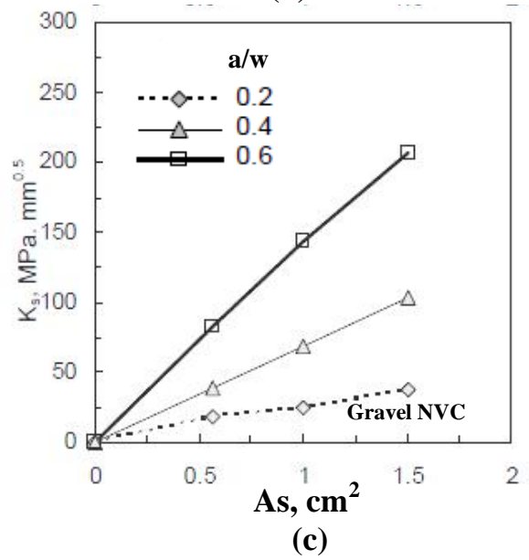
Fig. 8 Effect of area of steel on the closing SIF of NVC
