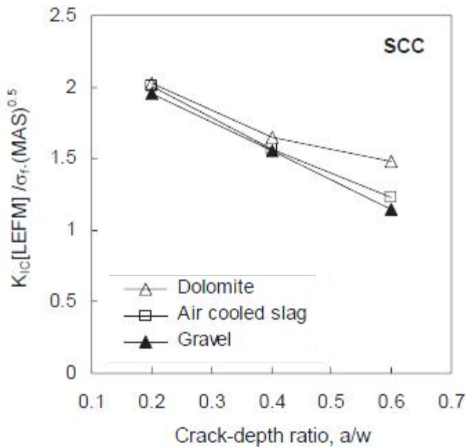
Fig. 1 Variation of K_{IC} based on LEFM concept with a/w for SCC
