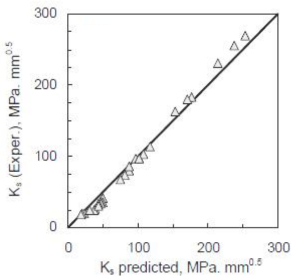
Fig. 9 Comparison between the experimental results and the predicted values of K_s for SCC beams.
