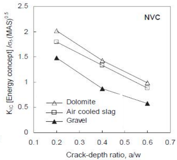
Fig. 4 Variation of K_{IC} based on energy concept with a/w for NVC
