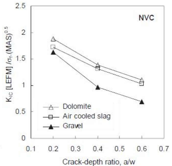
Fig. 2 Variation of K_{IC} based on LEFM concept with a/w for NVC
