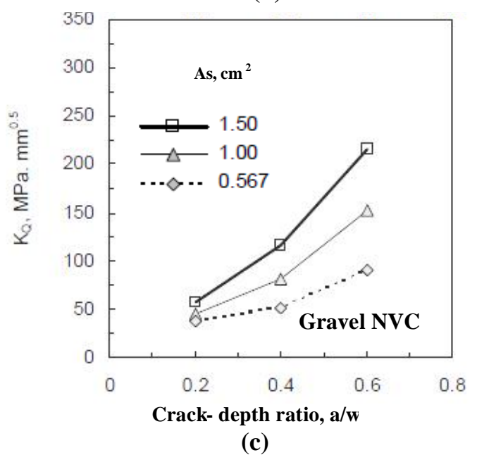
Fig. 6 Variation of K_{IC} with a/w for NVC reinforced concrete beams
