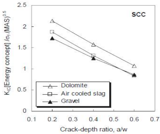
Fig. 3 Variation of K_{IC} based on energy concept with a/w ratio for SCC
