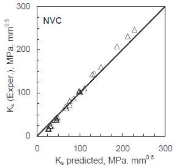
Fig. 10 Comparison between the experimental results and the predicted values of K_s for NVC beams
