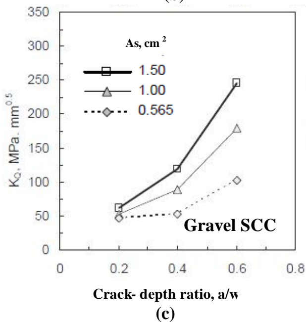
Fig. 5 Variation of K_{IC} with a/w for SCC reinforced concrete beams
