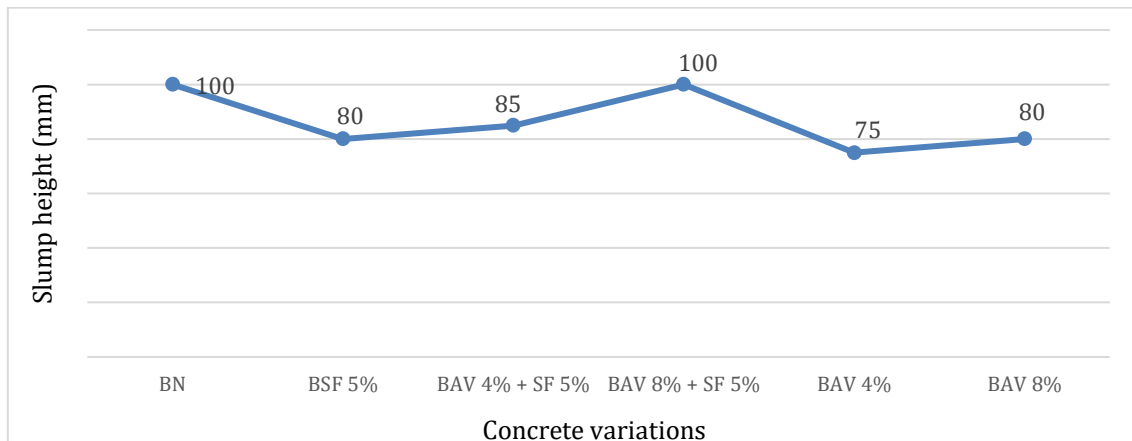
Fig. 5. Slump values of concrete specimens.
